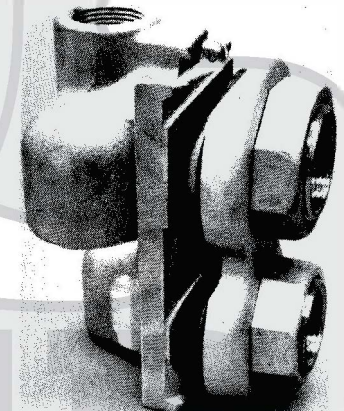
MHB400 Jet Pitless Adapter
